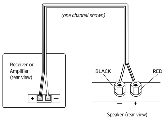
FIGURE 4 – Wiring diagram shows polarity connections for one channel of a stereo or home theater system.
